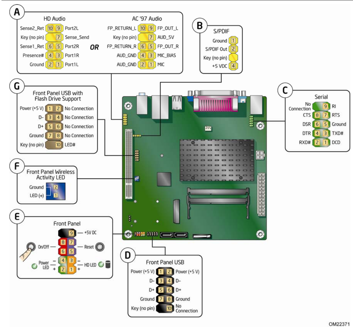
Figure 12. Internal Headers
